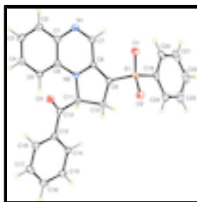
Fig. 1. Ellipsoids at the 50% level, with H atoms having arbitrary radius.
